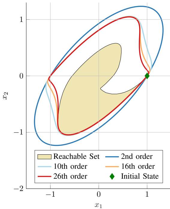
Fig. 1: Simulated system response of (18). When starting from x_0 = [1, 0]^T , the system can only reach the region shown in light yellow, which was computed via simulation. The dark blue, light blue, orange and red regions represent invariant sets calculated using quadratic, 10 th -order, 16 th -order and 26 th -order meta-Lyapunov functions, respectively. The invariance of these regions is shown by (19).
