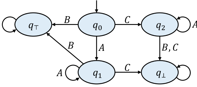
Figure 4. Monitor automaton \mathcal{M}^{\varphi_2} = (\Sigma, Q, q_0, \delta, \lambda) for the LTL property \varphi_2 = (\bigcirc A) \vee (A \cup B) evaluated over the alphabet \Sigma = \{A, B, C\} . States q_0, q_1 , and q_2 have output inconclusive , “?”. States q_\perp and q_\top have outputs false , “ \perp ”, and true , “ \top ”, respectively.
