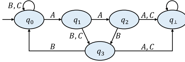
Figure 2. Monitor automaton \mathcal{M}^{\varphi_1} for the LTL specification \varphi_1 = (A \rightarrow \bigcirc^2 B) evaluated over the alphabet \Sigma = \{A, B, C\} . States q_0, \dots, q_3 have output inconclusive , '?', and state q_{\perp} has output false , \perp .
