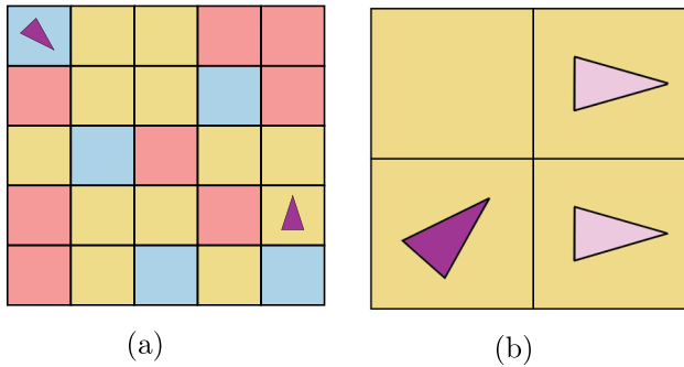
Figure 6. Problem setting. (a) shows the labelling of the system state space, and (b) describes the nondeterministic control actions.
