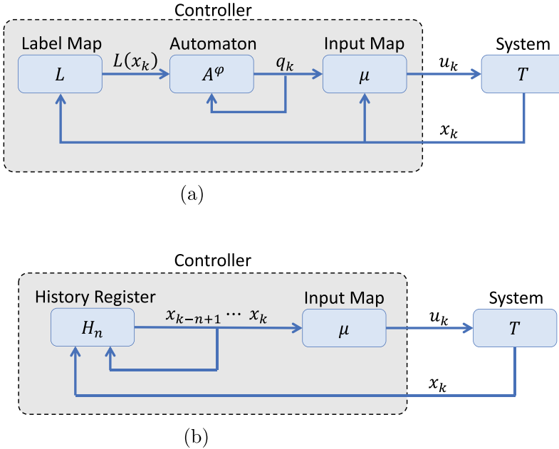
Figure 1. Two controller designs which assure the system T = (\mathcal{X}, \mathcal{U}, f, \Sigma, L) against the LTL specification \varphi .
