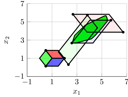
(a) The initial set \mathcal{X}_0 is the union of three disjoint parallelograms \mathcal{X}_0^1 , \mathcal{X}_0^2 and \mathcal{X}_0^3 , shown red, green and blue. The reachable set of each is approximated using theorem 1 and is shown in respective colors. The true reachable set R(1; \mathcal{X}_0) is shown in green.
