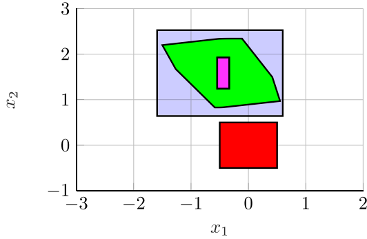
(b) Projection of Figure 2a onto the x_1 - x_2 plane.
