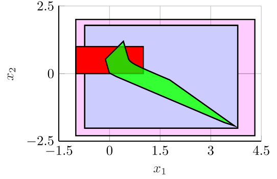
Fig. 1. Approximating forward reachable sets for (18) from the set of initial conditions \mathcal{X}_0 = [-1, 1] \times [0, 1] , shown in red. R(1; \mathcal{X}_0) is computed via exhaustive simulation and is shown in green. Hyperrectangular over-approximations of R(1; \mathcal{X}_0) are computed from (19) and [1, Th. 1] and are shown in blue and pink, respectively. 1
