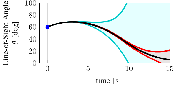
Fig. 6. Case Study: Computing reachable sets for (29)–(30) by applying Theorem 1 and Corollary 1. Two hyperrectangular over-approximations of R^\theta(t; x_0) are computed, with initial state x_0 = (q_0, \omega_0) given by (35). The over-approximation of R^\theta(t; x_0) attained from applying Theorem 1 with decomposition functions for (29) and (30) is shown in blue. The over-approximation of R^\theta(t; x_0) attained from applying Theorem 1 with the transformed first subsystem (36) is shown in red. Note that applying a linear transformation to the subsystem dynamics allows for higher fidelity reachable set computations. The initial state x_0 = (q_0, \omega_0) given by (35) is shown in blue, and the deterministic trajectory \theta(\Phi^F(t; x_0, 0)) , arising from the case with no disturbances, is shown in black.
