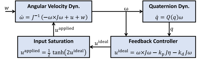
Fig. 5. Case Study: Depiction of the spacecraft model as an interconnection amongst subsystems.
