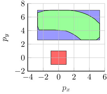
Fig. 3. Example 1: computing reachable sets for (26) by applying Theorem 1. A hyperrectangular over-approximations of R^F(6; A) is computed, with initial set A = [-1, 1]^2 \times [\frac{\pi}{3}, \frac{\pi}{2}] and where \mathcal{W} = [0.9, 1] \times [-0.1, 0.1] . The over-approximation of R^F(6; A) attained from applying Theorem 1 is shown in blue, projected onto the p_x - p_y plane. The initial set A is shown in red, and the true system reachable set R^F(6; A) , which was computed via exhaustive simulation, is shown in green.
