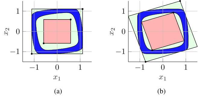
Fig. 2. Example 2: Computing robustly forward invariant sets for (23) by applying Theorems 1 and 2. (a) \mathcal{X}_{\text{eq}} is the larger rectangle and \mathcal{Y}_{\text{eq}} is the smaller rectangle. It follows from Theorems 1 and 2 that the shaded green region is robustly forward invariant and attractive for (23), and the complement of the red region is forward invariant for (23). The region shown in blue is the smallest attractive set computed numerically. (b) Larger parallelogram corresponds to an equilibrium in the embedding space of (26), and the smaller parallelogram corresponds to an equilibrium in the embedding space of the backward-time dynamics. The shaded green region is robustly forward invariant and attractive for (23), and the complement of the red region is also forward invariant.
