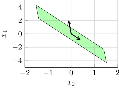
Fig. 3. Case Study 1: Invariant regions for the quadrotor model (31) under (33), projected onto the x_2, x_4 plane. The parallelogram [\underline{x}, \bar{x}]_T , with \underline{x} and \bar{x} from (39) is shown in green. Since 0 \preceq_{SE} e(\underline{x}, \bar{x}) , it follows from Theorem 1 that the green region is forward invariant for (31) under (33). Two eigenvectors of A , which are used to construct the transformation T , are shown as black arrows.
