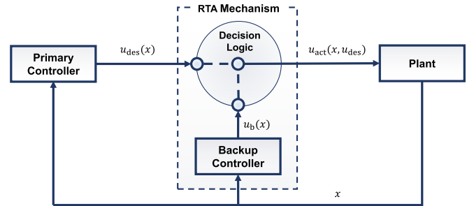
Fig. 1. Run time assured control system architecture. Control inputs u_{des} are suggested by a potentially unsafe primary controller, possibly a human operator. When necessary to preserve system safety, the RTA mechanism applies, instead, a known safe backup control input u_b to the plant. The backup controller is certified to be safe via the explicit knowledge of a forward invariant set and, in this way, system safety is ensured for all time.
