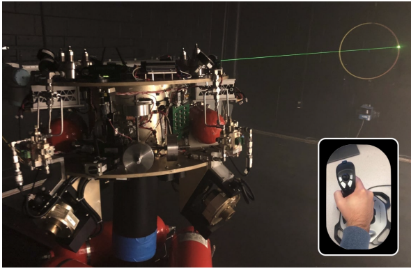
Fig. 6. Experimental setup: The inertially fixed \hat{K} vector is chosen to point toward a ring, with the border of the ring describing the extent of the unsafe set. A laser pointer is fixed to the body-fixed \hat{k} direction so that the laser touches the ring when \theta(x) = 175^\circ . Nominal, possibly unsafe, control actions are suggested by a human operator via a joystick.
