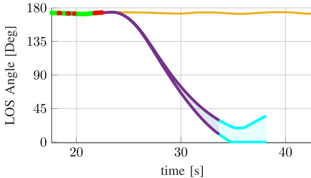
Fig. 8. In-the-loop reachability analysis: at time t = 22.5 s, the backup controller is applied due to a violation of the safety constraint. t_p + t_b = 15.6 s reachable set prediction is shown in light blue. If the backup controller is applied, the system is guaranteed to reenter the backup region \mathcal{C}_b in 11 s, as shown in purple.
