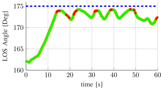
Fig. 7. Line-of-sight angle versus time. Green indicates time iterations that are unfiltered and red indicates times when the RTA filter is active. The extent of the admissible set, \theta_{\max} = 175^\circ , is shown in the blue dashed line.
