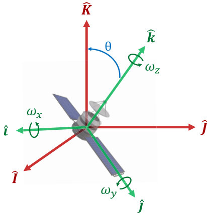
Fig. 2. Depiction of spacecraft system. The inertially fixed reference frame \mathcal{F}_I := (\mathcal{O}, \hat{i}, \hat{j}, \hat{K}) is shown in red and the body-fixed reference frame \mathcal{F}_B := (\mathcal{O}, \hat{i}, \hat{j}, \hat{k}) is shown in green. The line-of-sight angle, which is the angle made between the \hat{k} and \hat{K} directions, is given by (7) and is shown in blue. Note that the vectors \omega , u , and w in (5) are all taken with respect to \mathcal{F}_B .
