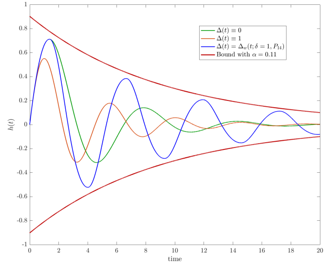
Fig. 2: Example 3. Impulse response plots showing how using the worst-case switching function can cause an impulse response to approach an exponential bound.
