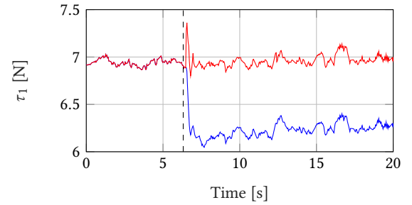
(b) Quadrotor 1 thrust command vs. experiment time.
