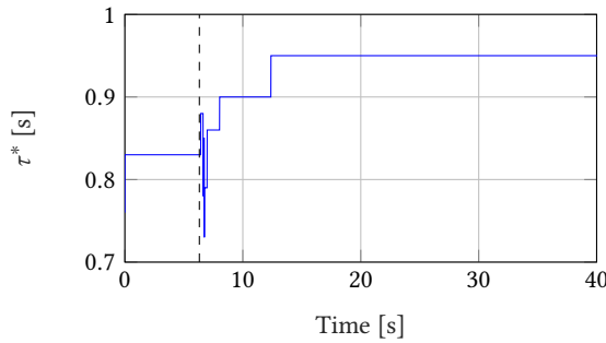
(b) Argument solution t^* for (21) vs. experiment time. At time t^* the systems reachable set under the backup control policy is contained within S_b
