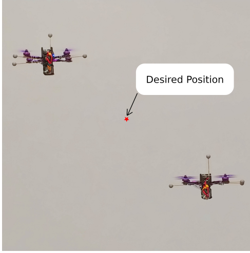
Figure 4: Photograph of the two quadrotors during the flight experiment. The vehicles are both commanded by an unsafe controller with a desired position that nominally results in a collision. The proposed RTA algorithm supervises the vehicles and filters the unsafe controller resulting in a safe displacement while the vehicles are centrally positioned at the desired unsafe position.
