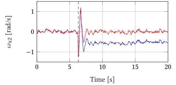
(c) Quadrotor 2 roll rate command vs. experiment time.
