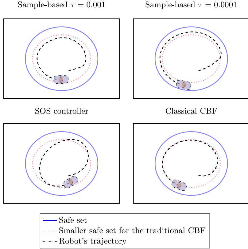
Fig. 3. Trajectories for the sample-based controller with \tau = 0.001 and \tau = 0.0001 , as well as the SOS controller and the traditional CBF controller. The boundary of the safe set in the workspace is shown in solid blue. The traditional CBF controller must use a smaller safe set in the statespace to accommodate the system's extent; the boundary of this smaller set is shown in dotted red. The plots demonstrate that conservatism of the sampling-based approach decreases as \tau decreases and the number of samples increases. Moreover, due to the non-circular shape of the extent set, the traditional CBF controller is more conservative compared to both the sample-based controller with \tau = 0.0001 and the SOS controller.
