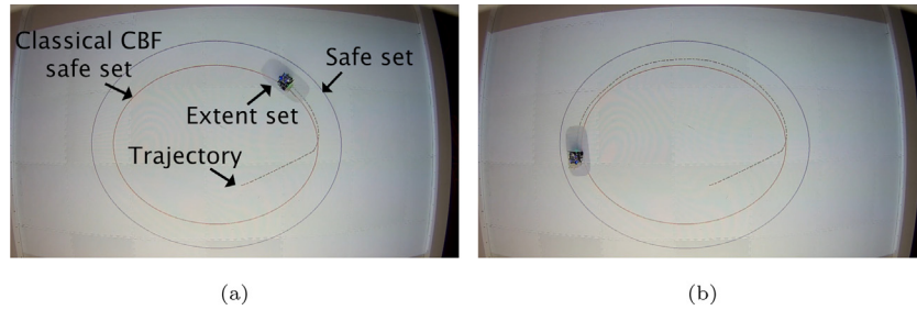
Fig. 5. Overhead images from the implementation on the Robotarium test-bed. Each of the sub-figures indicate the trajectory of the robot generated over the course of the implementation. Observe that although the nominal controller tries to push the robot outside the safe set, the sampling-based controller (12) ensures that the robot state and its extent stay within the safe set.
