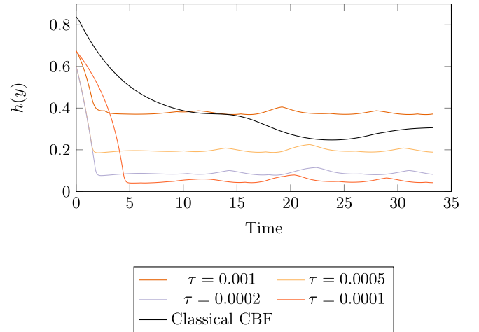
Fig. 4. Minimum value of the Ec-CBF h(y) evaluated for \tau = 0.001 , \tau = 0.0005 , \tau = 0.0002 , and \tau = 0.0001 at the sampled points (i.e. for all y \in \partial \mathcal{E}_\tau(x) ) on the boundary of the extent set. Observe that all values for each case are strictly positive, thus implying that none of the sampled points cross into the unsafe region. For comparison, the classical CBF solution is included that uses a smaller safe set. The classical solution is more conservative than almost all of the sample-based solutions.
