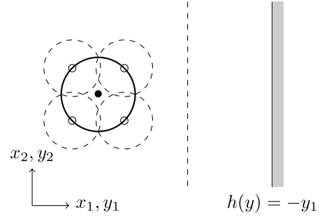
Fig. 2. Example of the different discretizations in Example 1. The black dot is the system and the solid circle its extent. The four discretization points are with circles and the distances with dashed circles. The dashed line show how close the discretizations points can be to the barrier and still satisfy the inequality.
